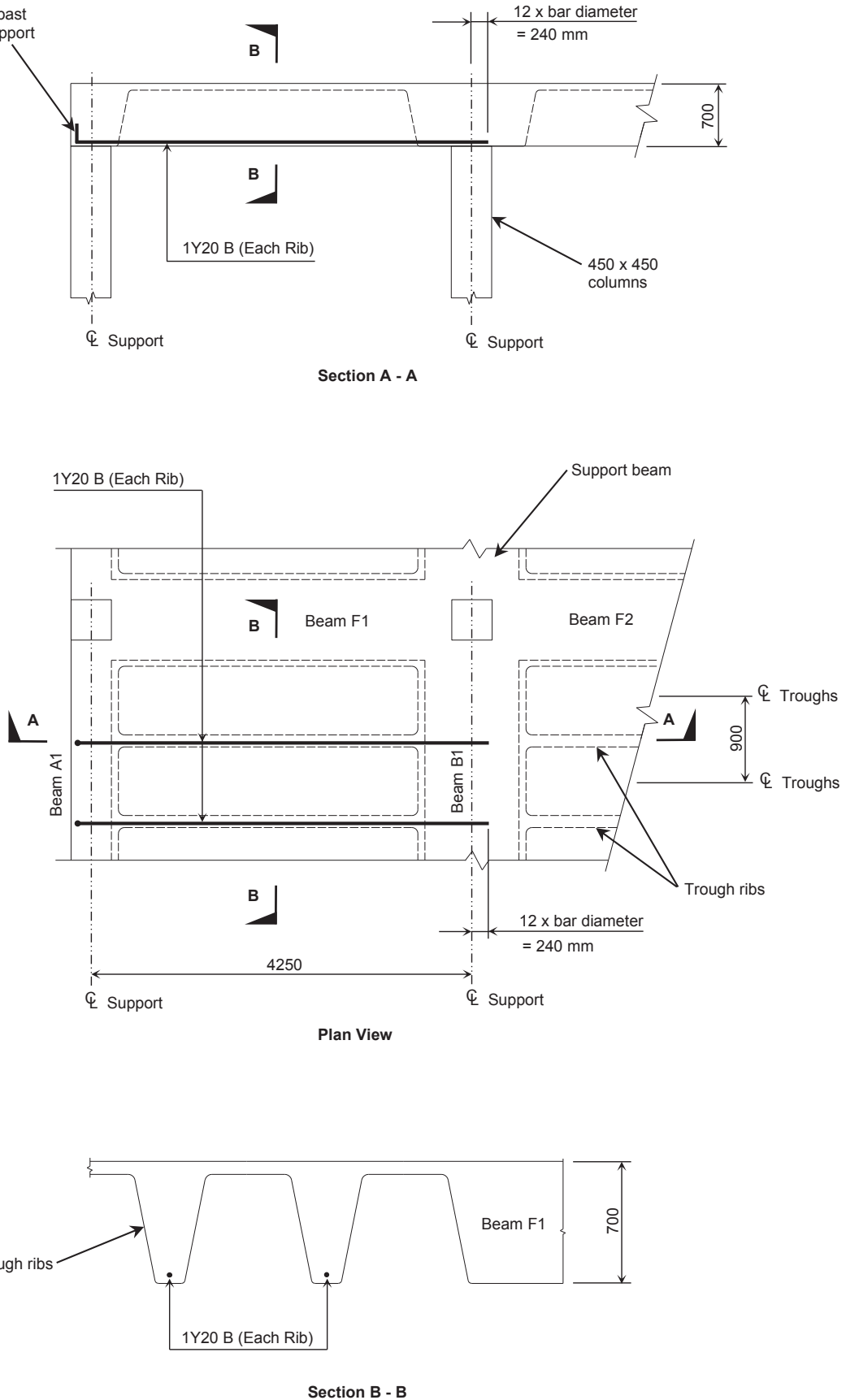
Figure 32 – Bottom Tension Reinforcement For Trough Ribs
