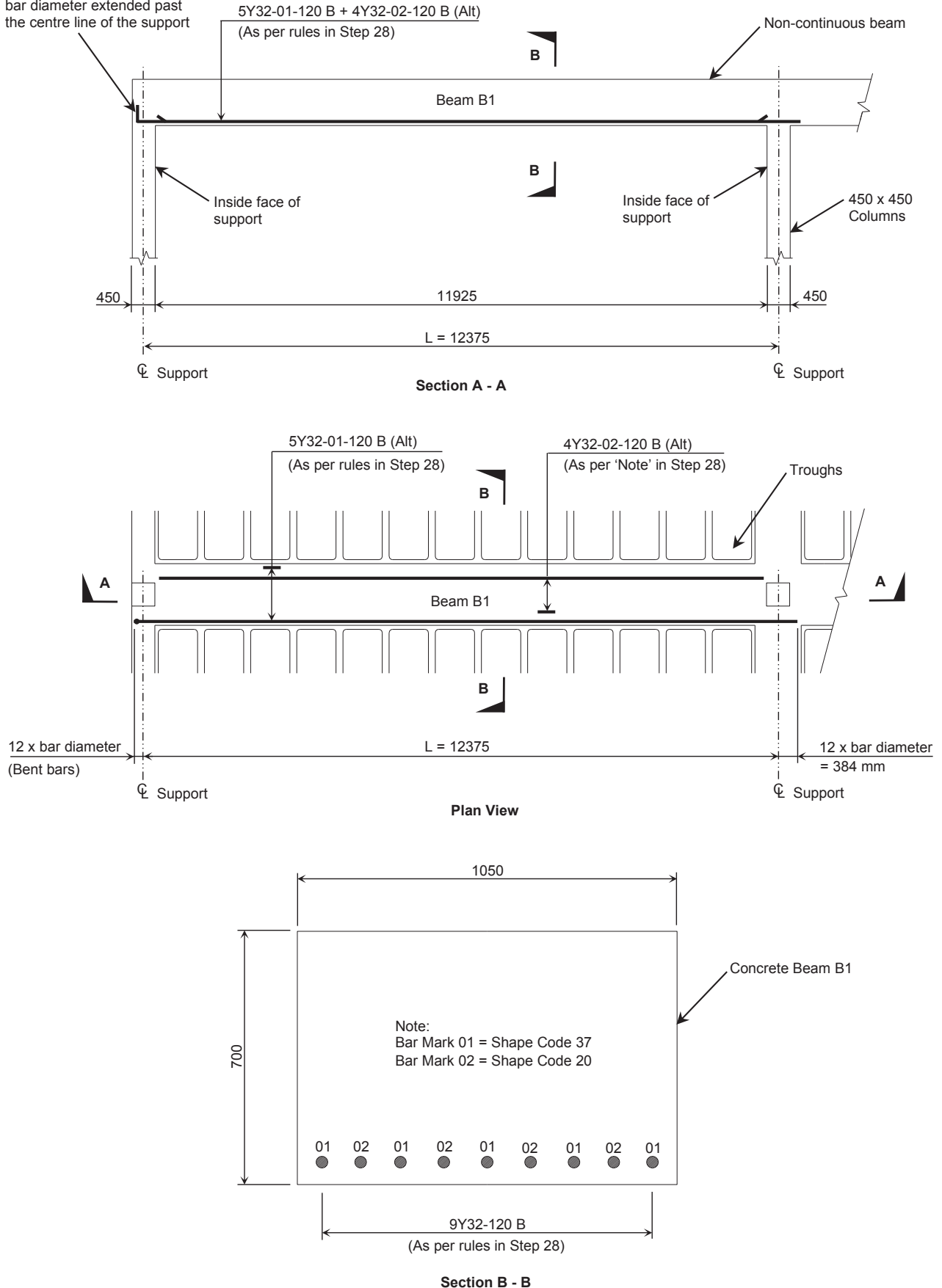
Figure 27 – Bottom Tension Reinforcement For Beam B1
