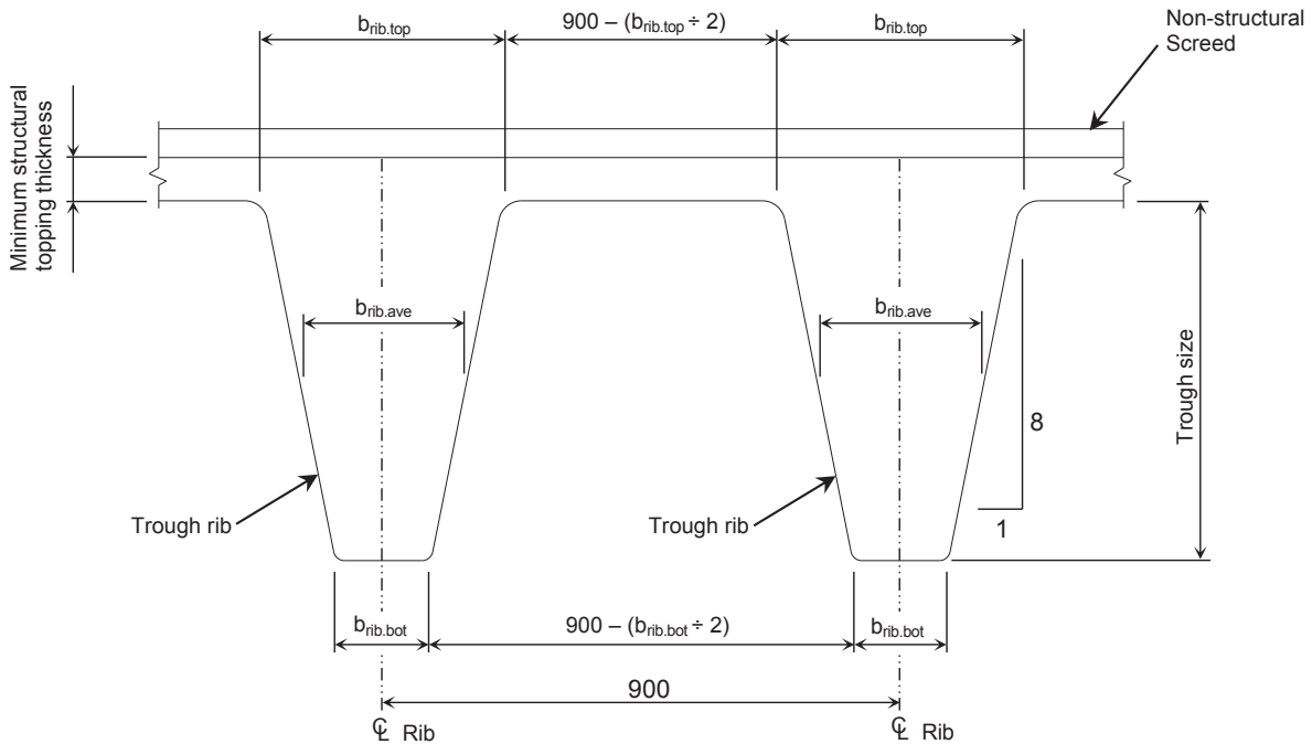
Figure 24 – Typical Trough Section
