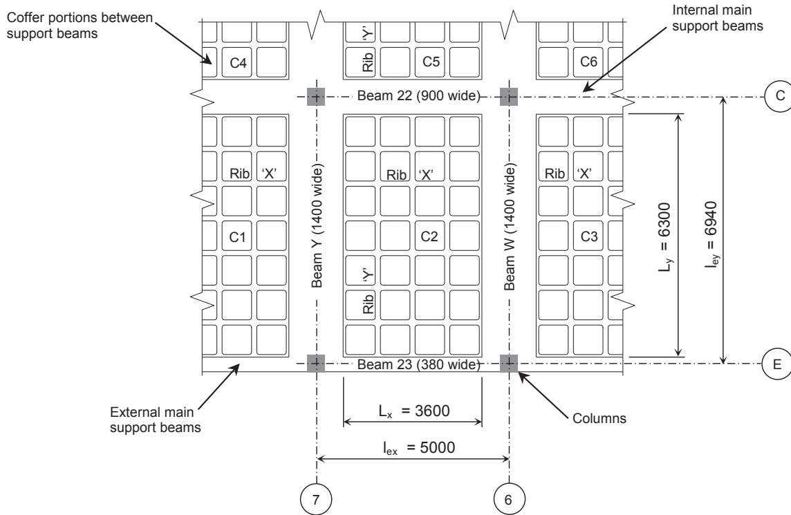
Figure 13 – Typical Beam And Coffers Layout Showing Various Coffer Portions Between Support Beams (Extract From Figure 3)
